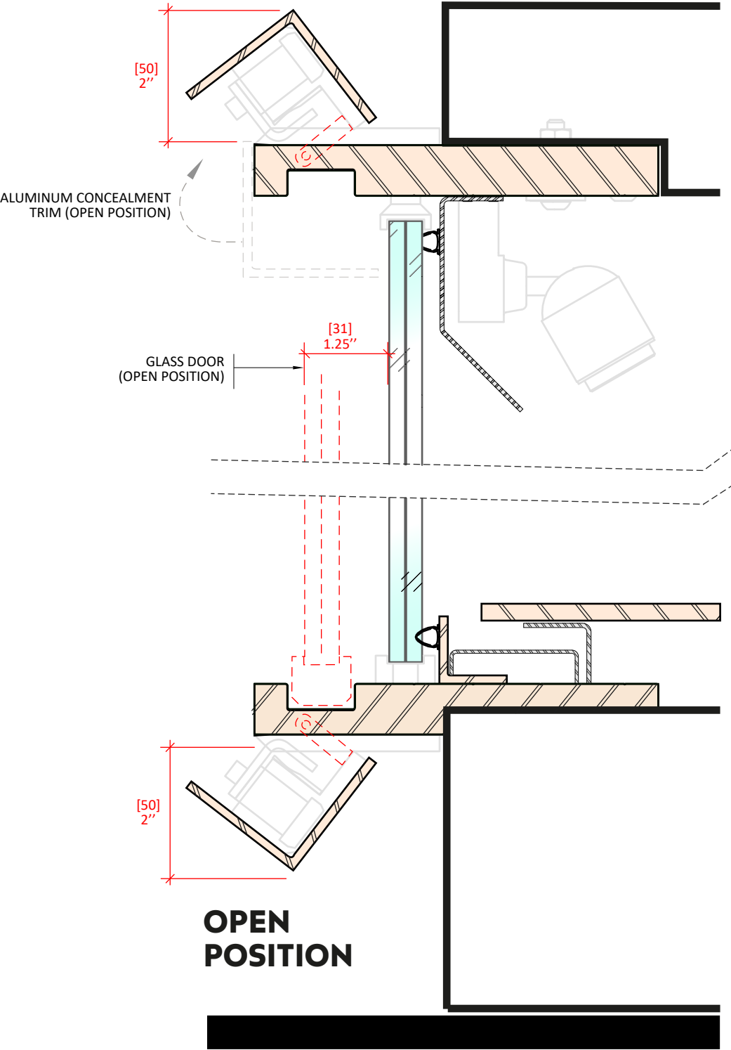
TYPICAL SECTION SCALE 1:2
