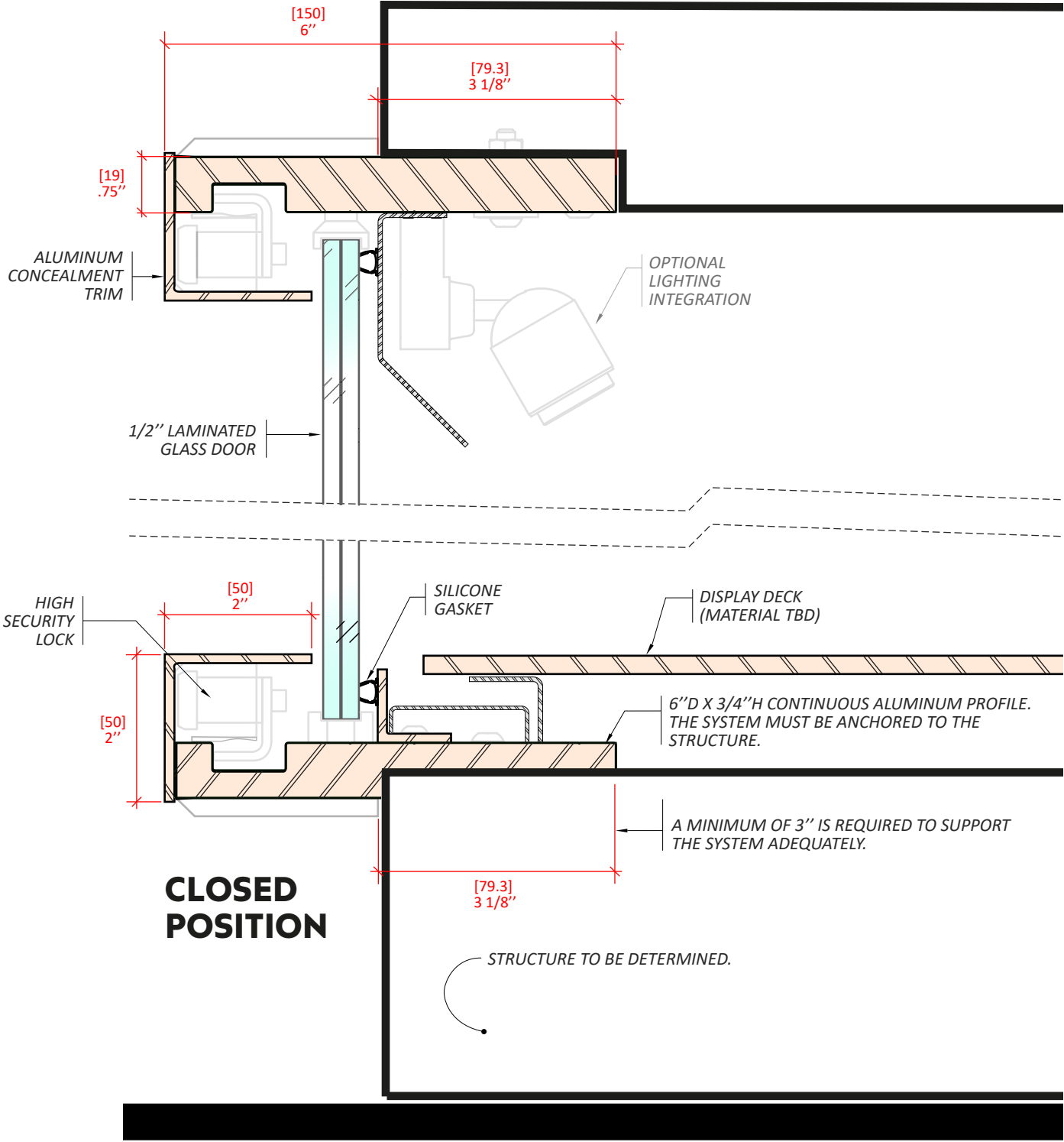
TYPICAL SECTION SCALE 1:2
